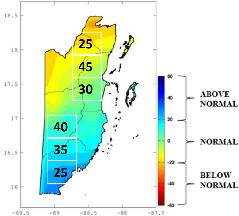
RAINFALL FORECAST: DJFM 2017-2018 (mm) (%ABOVE/BELOW AVERAGE)
