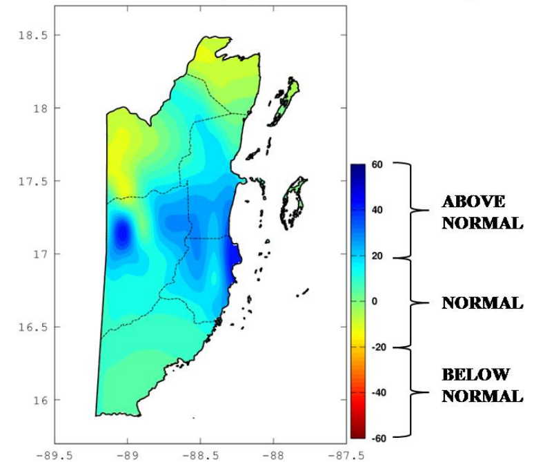
RAINFALL OBSERVED: DJFM 2017-2018 (mm) (%ABOVE/BELOW AVERAGE)
