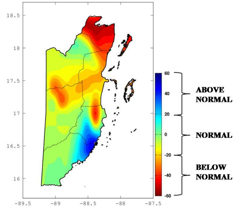
RAINFALL OBSERVED: DECEMBER 2017 (%ABOVE/BELOW AVERAGE)
