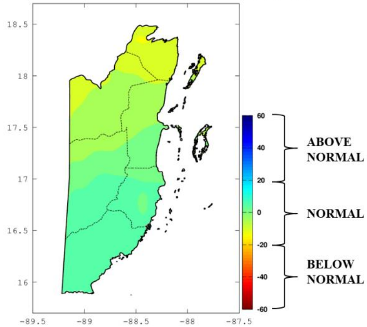
RAINFALL FORECAST: DECEMBER 2017 (%ABOVE/BELOW AVERAGE)
