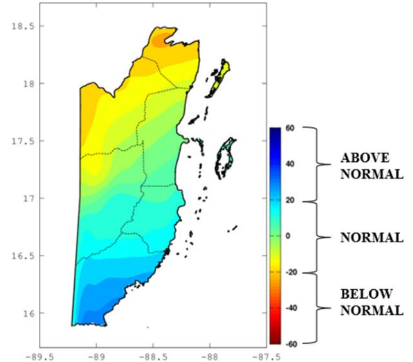
RAINFALL FORECAST: DJFM 2017-2018 (mm) (%ABOVE/BELOW AVERAGE)
