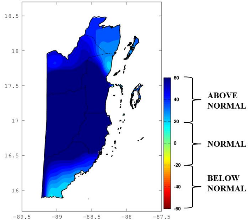
RAINFALL OBSERVED: FEBRUARY 2018 (%ABOVE/BELOW AVERAGE)
