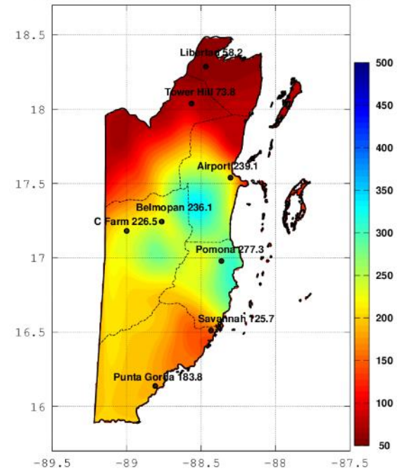
RAINFALL OBSERVED: JANUARY 2018 (mm)
