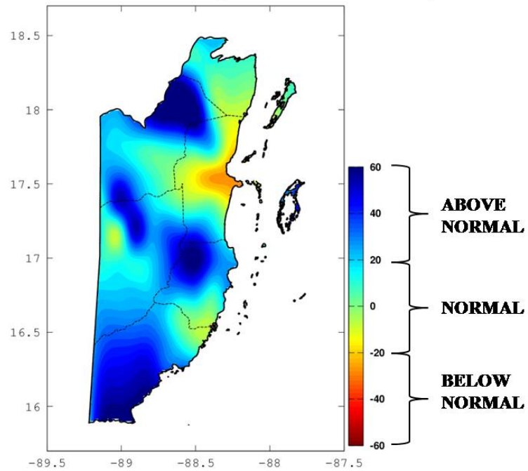
RAINFALL OBSERVED: APRIL 2018 (%ABOVE/BELOW AVERAGE)
