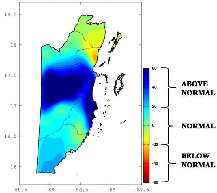
RAINFALL OBSERVED: JANUARY 2018 (%ABOVE/BELOW AVERAGE)
